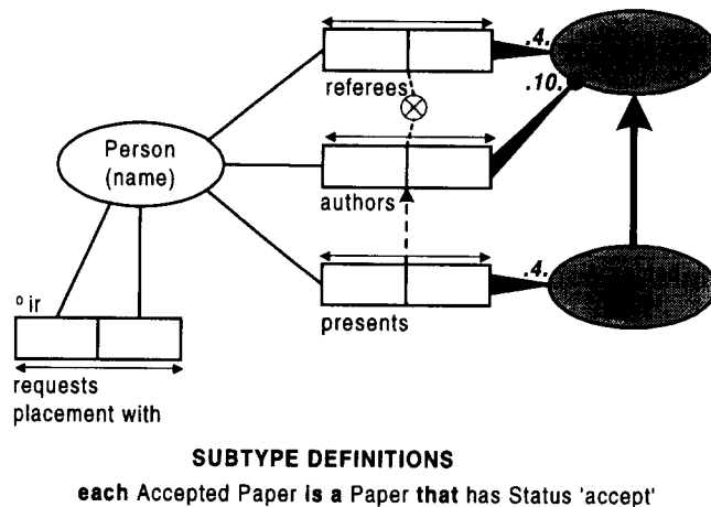
Fig. 35. WeightSchema( \mathcal{CS}_4 ): Abstraction level 4.
