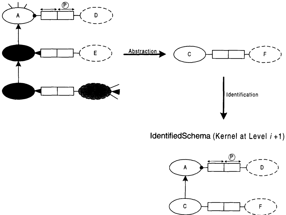
Fig. 27. The primary identification of subtype C is inherited from supertype A.
