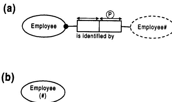
Fig. 4. (a) Explicit identification scheme; (b) implicit identification scheme.
