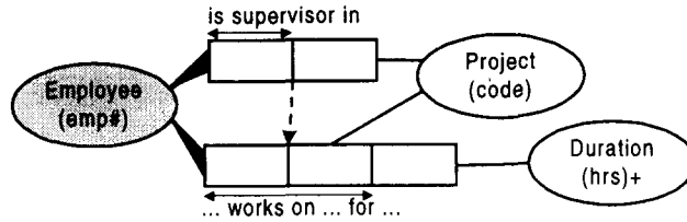
Fig. 18. Roles connected by multi-role set constraints are anchored.
