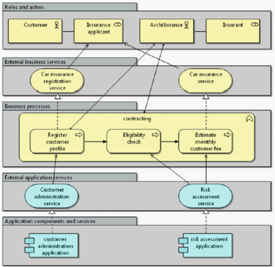
Fig. 24.4 ArchiSurance direct-to-customer enterprise architecture model © 2013 IEEE. Reprinted, with permission, from Plataniotis et al. (2013a)
